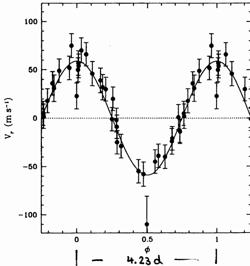
Figure 2. The variation of the radial velocity of 51 Peg (from Mayor M and Queloz D 1995 Nature 178 355).
